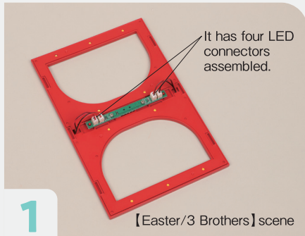
The Ceiling with four LED connectors assembled and Inner Panels assembled on both sides is for the 【Easter/3 Brothers】 scene.
