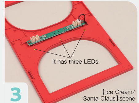
There are two Ceilings with LEDs fitted into one side. The one with three LEDs in the position shown is for the 【Ice Cream/Santa Claus】 scene.
